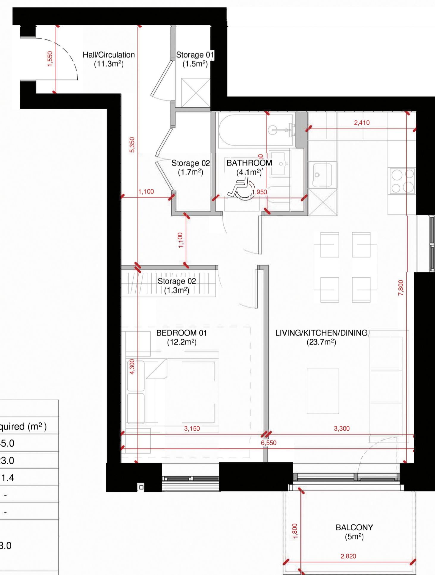
Apartment Type D03 Scale 1:50@A1
