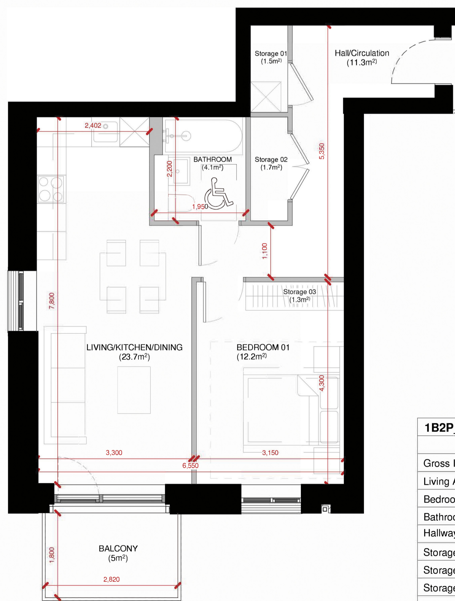
Apartment Type D02 Scale 1:50@A1
