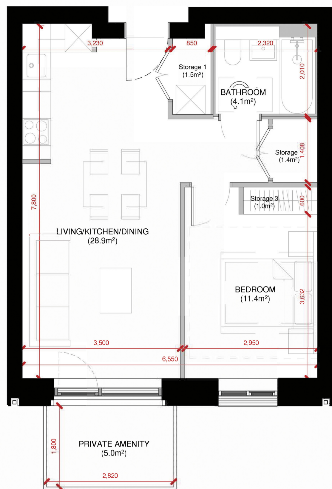
Apartment Type D01 Scale 1:50@A1
